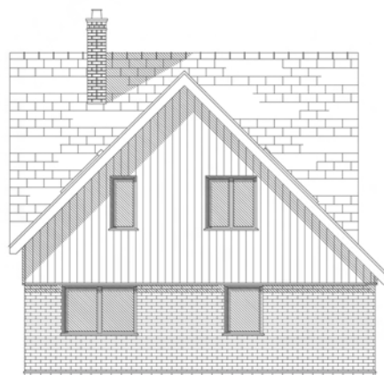
East Elevation
